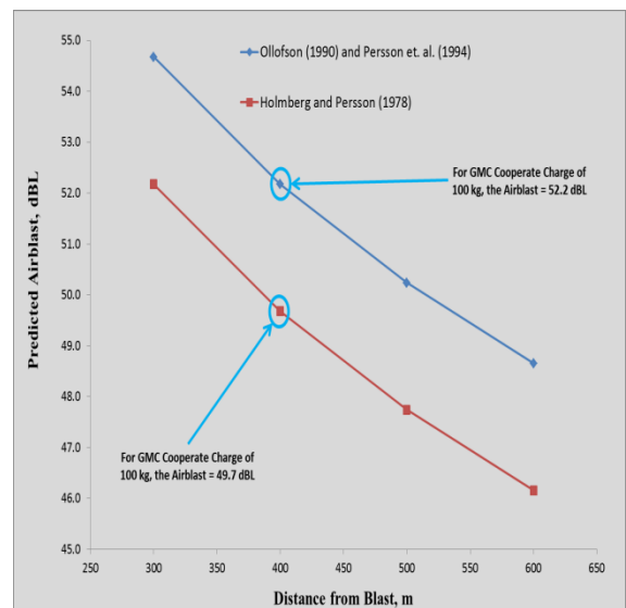
Fig. 6 Air blast Prediction Models at Pit C North
